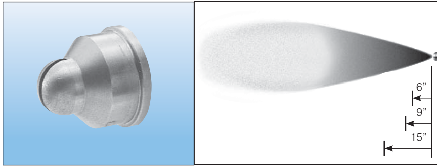
JPD Round Spray Performance Chart
